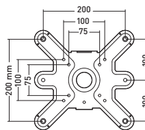
Platine TV
